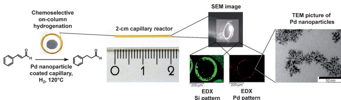
Figure 2. On-column hydrogenation over highly active Pd nanoparticles. Capillaries only 2 cm long coated with Pd nanoparticles stabilized in a polysiloxane matrix were used as the reactor. SEM and Si/Pd EDX (16 h) measurements show the coating of the fused silica microcapillaries (i.d. 250 \mu\text{m} , film thickness 0.25 \mu\text{m} ).
