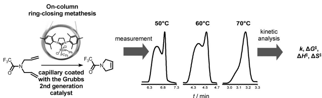
Figure 3. On-column metathesis over the Grubbs 2nd generation catalyst. In these experiments catalytic activity and separation selectivity is combined in a single 10-m-long capillary by dissolving the catalyst in the stationary separation phase. The elution profiles obtained were characterized by a pronounced conversion profile from the substrate to the product. Kinetic analysis was performed directly with the unified equation from Ref. [8].
