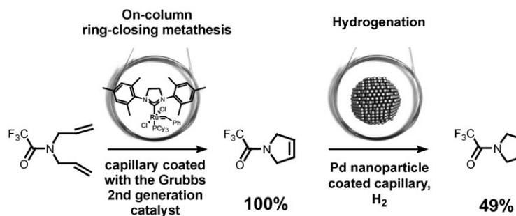
Figure 4. Modular design for a two-step on-column cascade reaction. N -trifluoroacetylpyrrolidine was synthesized within 6 min by coupling a 80 cm long metathesis column and a 10 cm long Pd nanoparticle hydrogenation column. H 2 was used as the reactive carrier gas.
